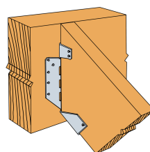
Sloped connection.
