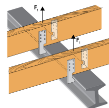
Attached timber joist to IPN with 2 AI
