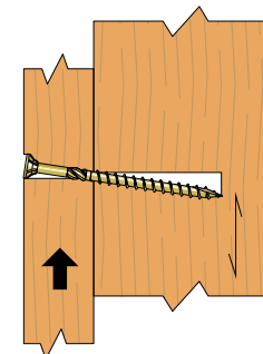
3. Double compression
