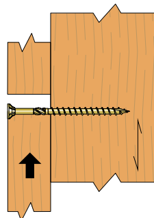
2. Compression timber 1
